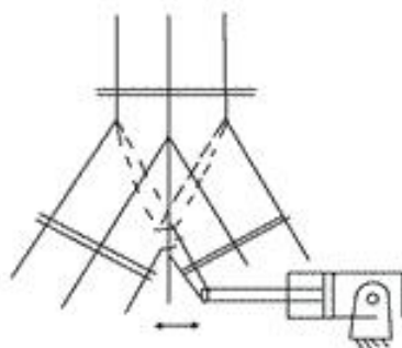
A 操纵三通管挡板换向
